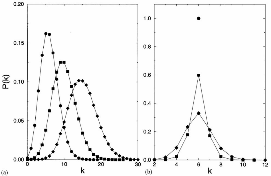
Fig. 2. Connectivity distributions for the ER and WS models. (a) P(k) in the ER model for N = 10000 and for p_{ER} = 0.0006 (circles), p_{ER} = 0.001 (squares) and p_{ER} = 0.0015 (diamonds). (b) P(k) in the WS model for N = 10000 , \langle k \rangle = 6 and three rewiring probabilities p_{WS} = 0 (circle, corresponding to the delta-function \delta(k - 6) ), p_{WS} = 0.1 (squares) and p_{WS} = 0.3 (diamonds).
